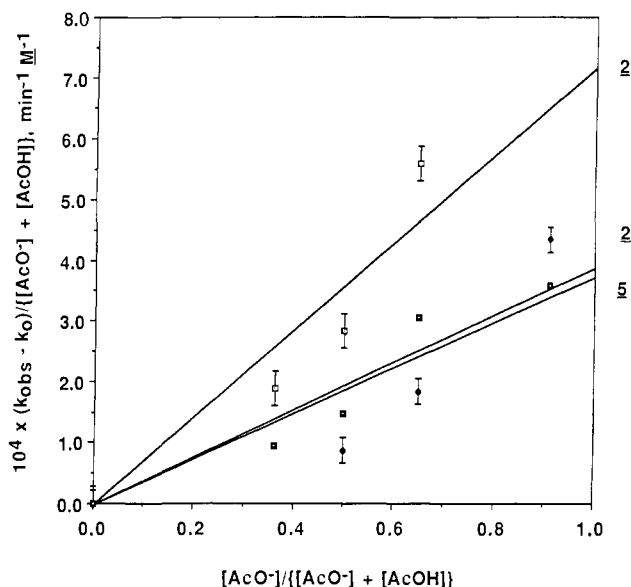
Figure 5. Dependence of the buffer-catalyzed hydrolysis rate of 2 ( \square , k_0 determined by extrapolation of k_0 obtained at higher pH values; \square , k_0 determined by extrapolation of rates in acetate buffer to zero buffer concentration; see text and Table III) and 5 ( \blacklozenge ; k_0 = 0 ) on the [\text{AcO}^-]/([\text{AcO}^-] + [\text{AcOH}]) ratio. Lines drawn are computer-generated best-fit lines through the experimental points.
