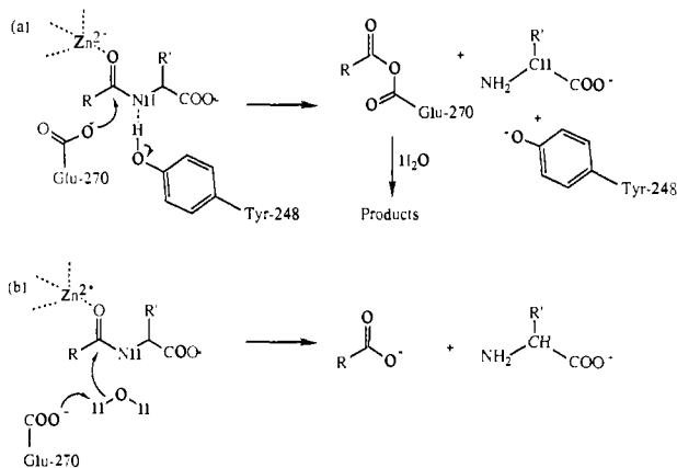
Scheme V
