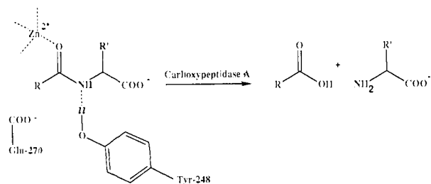
Figure 1. Schematic representation of CPA active site with bound glycy-L-tyrosine. 6
