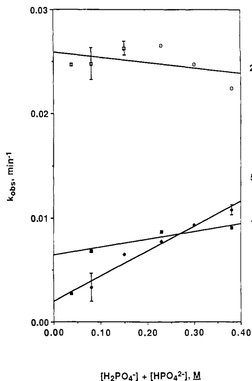
Figure 6. Plot of the observed pseudo-first-order rate constant for hydrolysis of 1 ( \blacksquare ), 2 ( \circ ), and 5 ( \blacklozenge ) vs. the concentration of phosphate buffer. Lines drawn are computer-generated best-fit lines through the experimental points.
