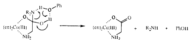
Scheme IX
